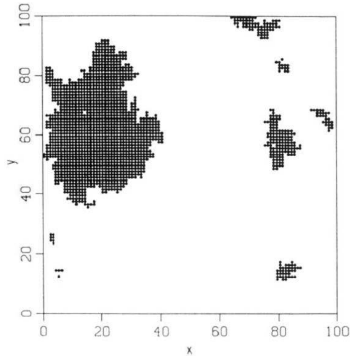
Figure 4. Domain structures resulted from several local perturbations in a 100x100 simulation array, with each cluster triggered by a single perturbation. From Bak, Tang and Wiesenfeld [1].
