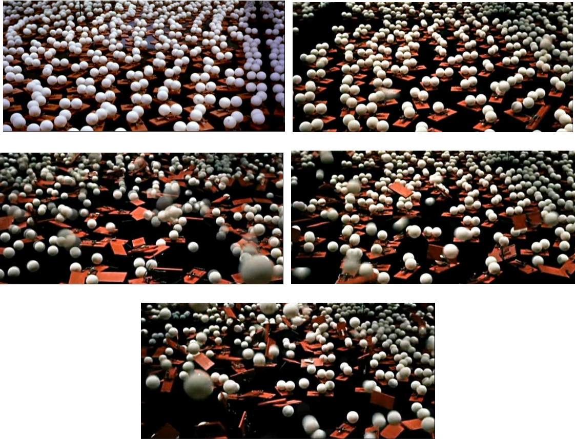
Figure 5. A just-critical system of mouse traps loaded with ping pong balls can turn supercritical with a single input perturbation. Source: Walt Disney.
