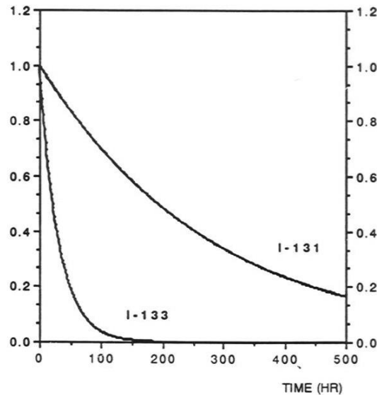
Figure 48. Decay curves of two short lived fission product isotopes, I 131 and I 133 .
