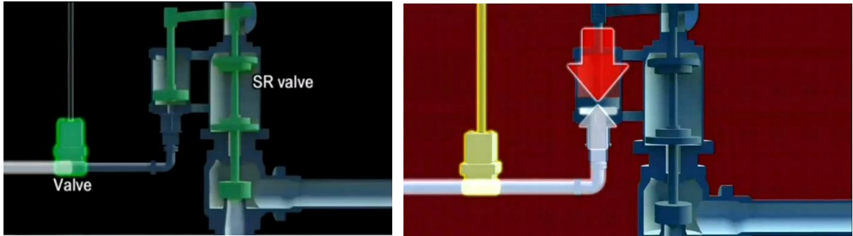
Figure 20. Battery-operated auxiliary valve releases nitrogen pressure to open safety relief valve to vent the containment of hydrogen and steam failed to operate because of unexpected high pressure in the containment that countered the nitrogen pressure. Operators tried to use connected car batteries to operate it unsuccessfully.
