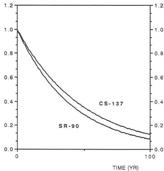
Figure 49. Decay curves of the two long lived fission product isotopes, Cs 137 and Sr 90 .
