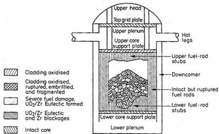
Figure 73. Debris bed resulting from the core damage in the Three Miles Island accident.
