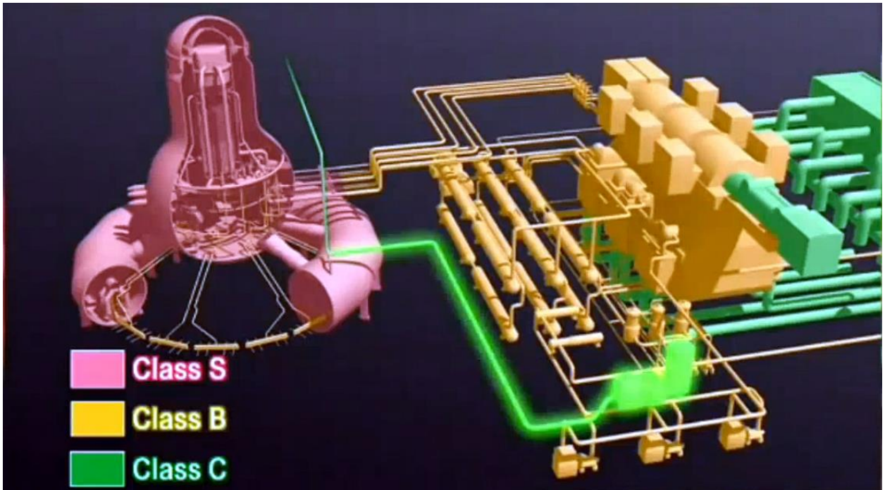
Figure 25. Seismic class C air duct to venting valve may have sustained cracks as a result of the earthquake.
