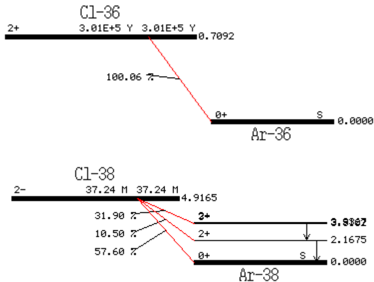
Figure 72. Decay diagrams of the Cl 36 and Cl 38 isotopes.
