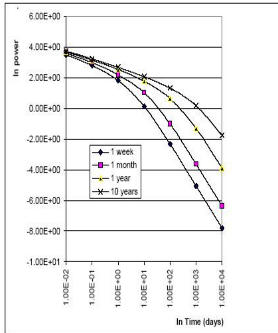
Figure 38. Decay heat power release for a 3,000 MWth Light Water Reactor, LWR for different operational times. The decay heat generation power decreases rapidly within a few days after shutdown.
