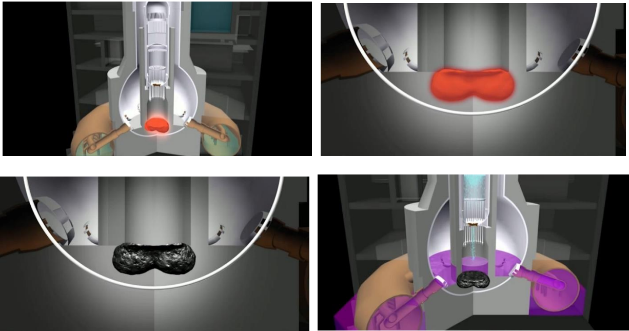
Figure 43. Molten corium material leaked through the control rods graphite seals into the dry well in the primary containment vessel. Dry well flooded through water injection from the top of the core. Source: Tepco.
