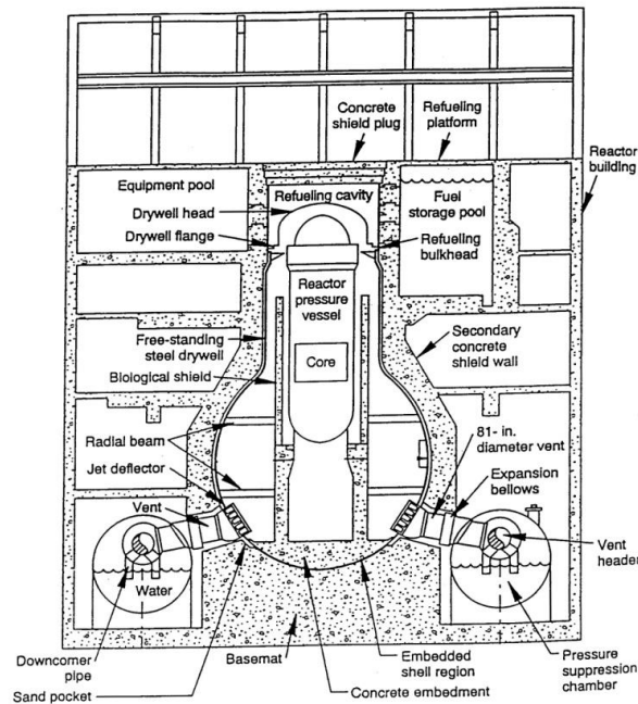
Figure 40. Primary and secondary containments configuration at Fukushima plants.
