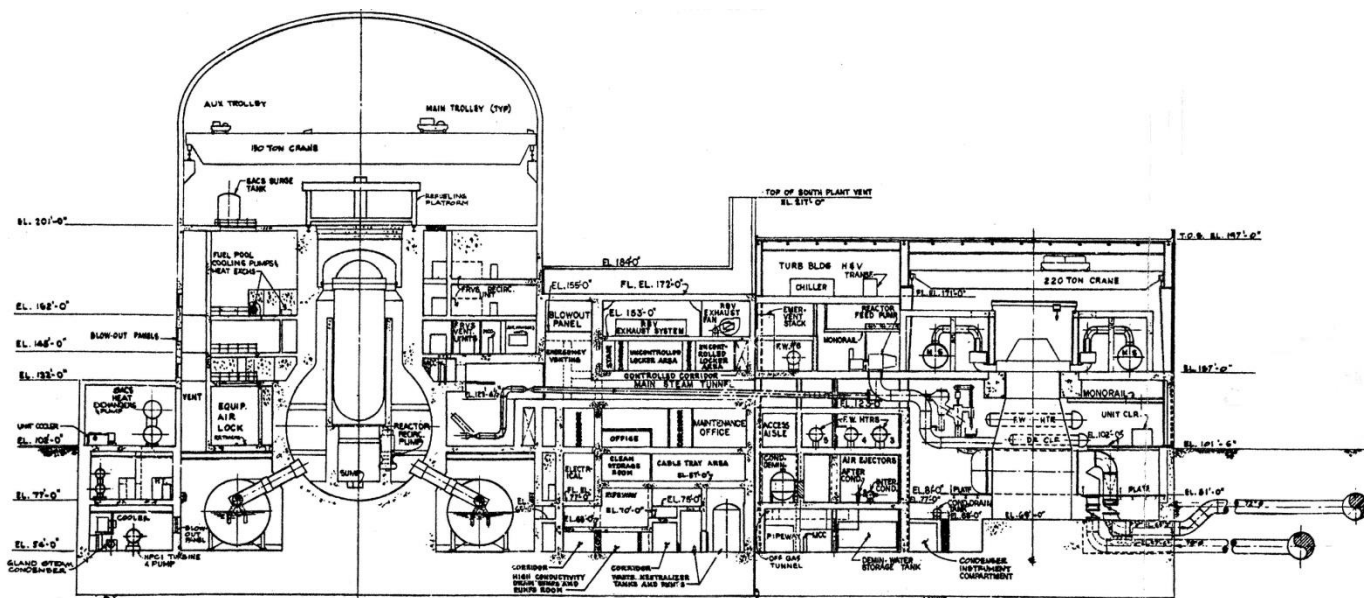
Figure 45. Cutout through containment and turbine hall showing the location of the fuel storage pool in a typical BWR. Plant systems below grade level and hence affected by flooding from the tsunami event include pumps and electrical components. The dry well includes a sump. Any leaking corium material through the control rod seals could interact with the sump water as well as the concrete mat causing a steam explosion, then becoming embedded in the concrete. Source: GE.
