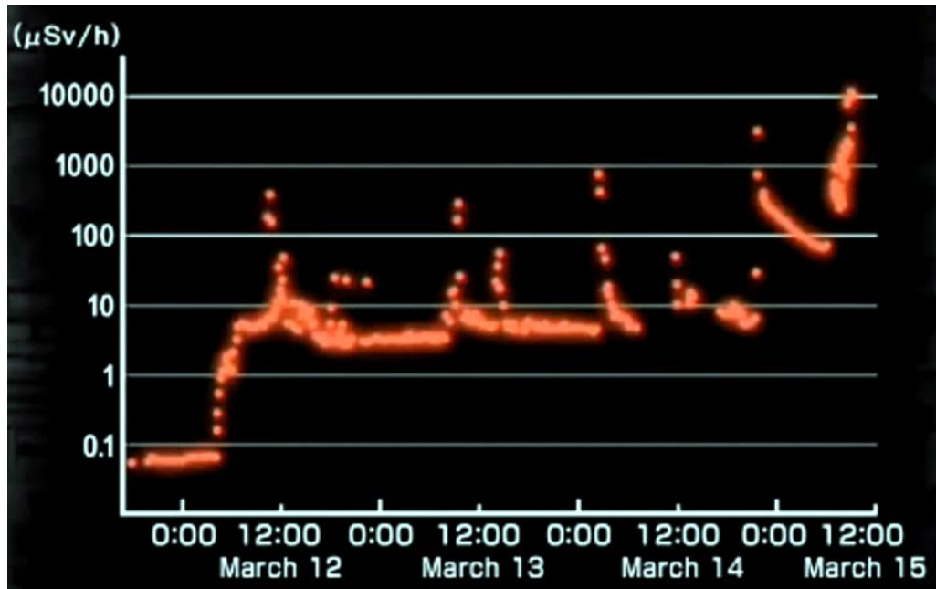
Figure 64. Dose equivalent rate at main gate of Fukushima Daiichi plants.
