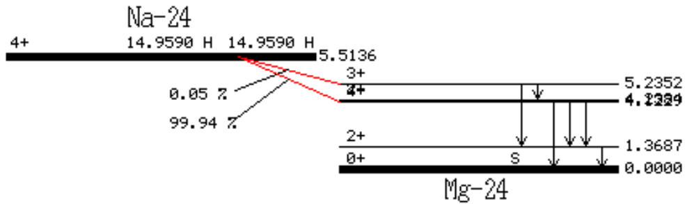
Figure 71. Decay diagram of Na 24 .
