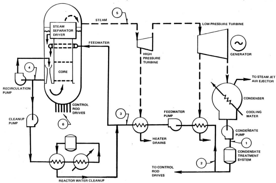
Figure 10. Typical BWR flow diagram. The role of the core spray system in the progression of the accident is undetermined. Source: GE.
