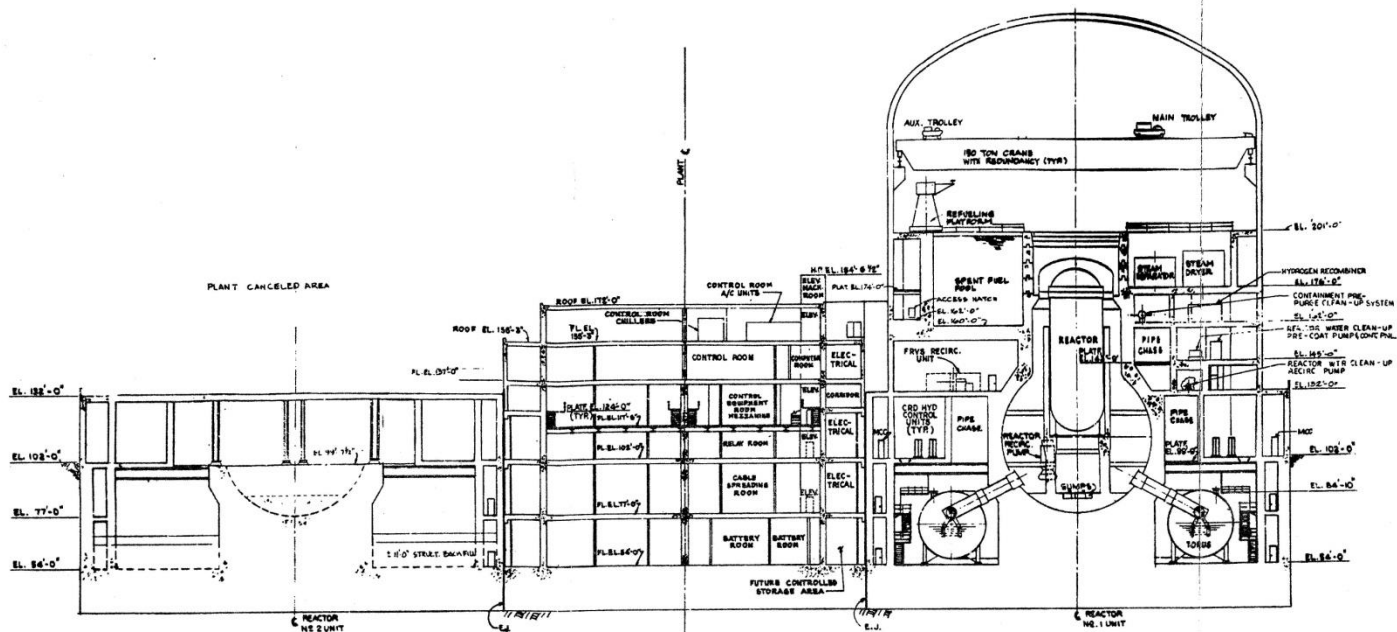
Figure 46. Perpendicular cutout through the containment structure showing the location of the storage batteries. The gate and other connections between the fuel storage pool and the top of the core may have sustained damage as a result of the earthquake and caused leakage of the pools' cooling water. Source: GE.
