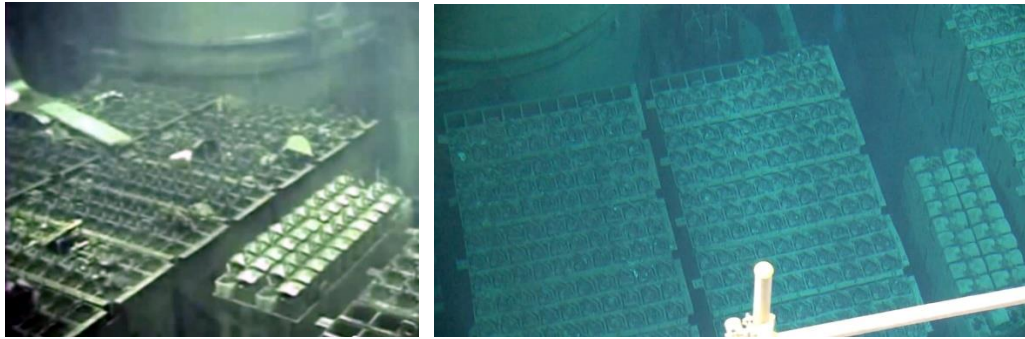
Figure 95. Debris removal in from unit 4 fuel storage pool.
