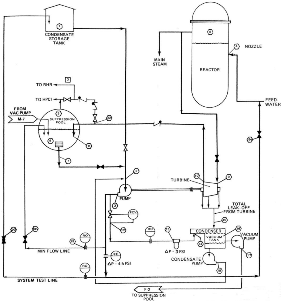
Figure 14. BWR Reactor Core Isolation Cooling system, RCIC. A steam turbine uses steam to drive a pump injecting water drawn from the condensate storage tank into the core. Exhaust from the steam turbine is directed to the pressure suppression pool. HPCI: High Pressure Coolant Injection system, RHR: Residual Heat Removal system.
