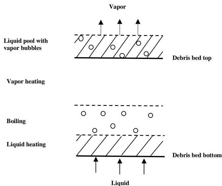
Figure 76. Multilayered once-through debris bed cooling.
