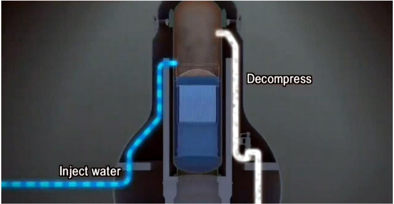
Figure 41. Depressurization of reactor vessel to allow Low Pressure Coolant Injection (LPCI) System to inject water at a high rate into reactor vessel..
