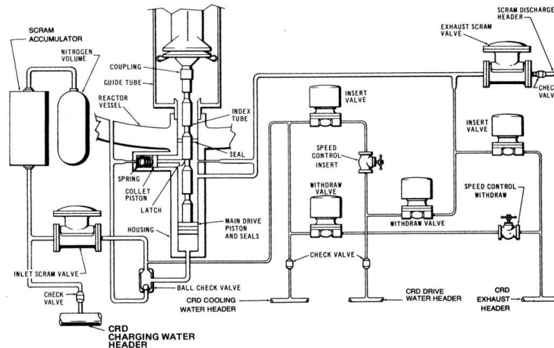
Figure 63. BWR control rod drive mechanism at the bottom of a BWR reactor vessel showing the control rod graphite seals location [2].
