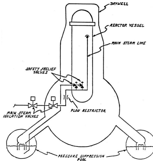
Figure 13. Main isolation valves and safety relief valves used in depressurization of the BWR. Source: GE.
