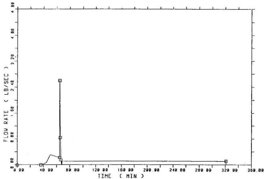
Figure 61. Hydrogen release rate was correlated with a pressure pulse inside the containment structure in the Three-Mile Island Accident. The hydrogen pulse did no discernible damage to the containment structure.
