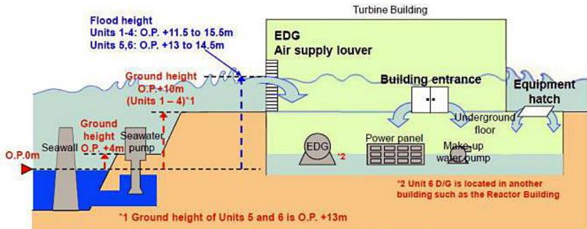
Figure 9. Inundation paths of major buildings at Fukushima plants.
