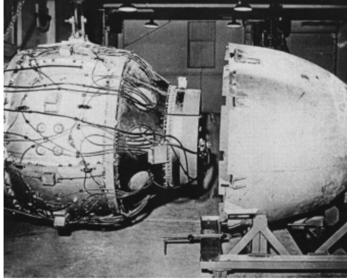
Figure 41. Disassembled Fat Man Implosion device dropped on Nagasaki. Fat Man used 6.4 kgs of Pu239 with a yield of 21 kT of TNT equivalent, whereas the less efficient Little Boy device used 64 kgs of U235 with a yield of 15 kT of TNT equivalent.
