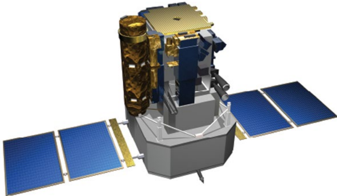
Figure 28. The SOHO satellite studies the sun from its deep core to the outer corona and the solar wind. It is 25 feet in width, weighs 2 tons and was launched in 1995. Source: NASA.
