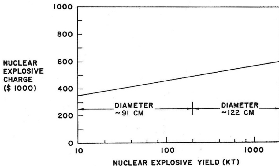
Figure 82. Charges for different yield charges in 1985 dollars. Source: USDOE.
