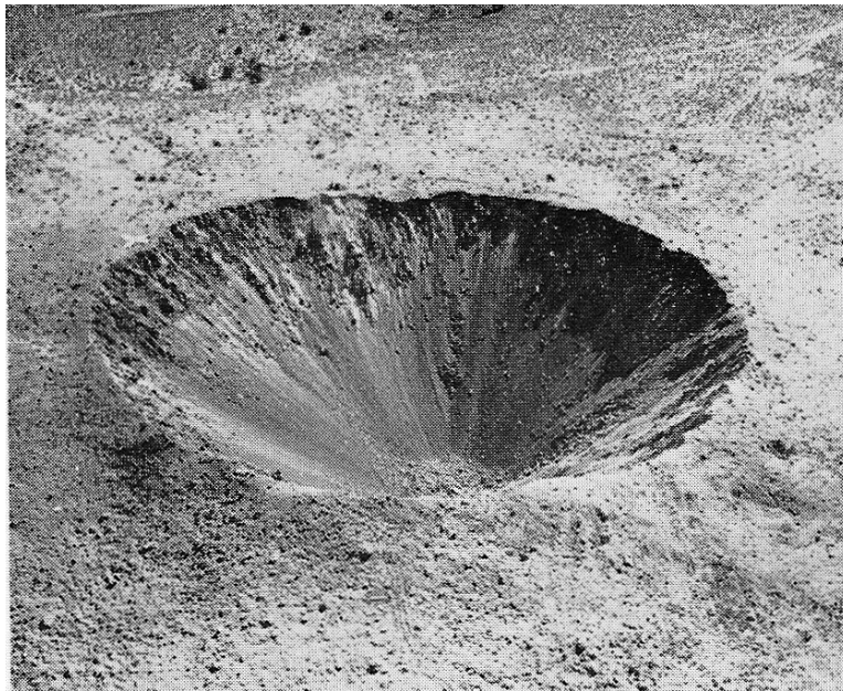
Figure 78. Cabriolet 2.3 kT TNT single shot experiment in basalt. Source: LLNL.
