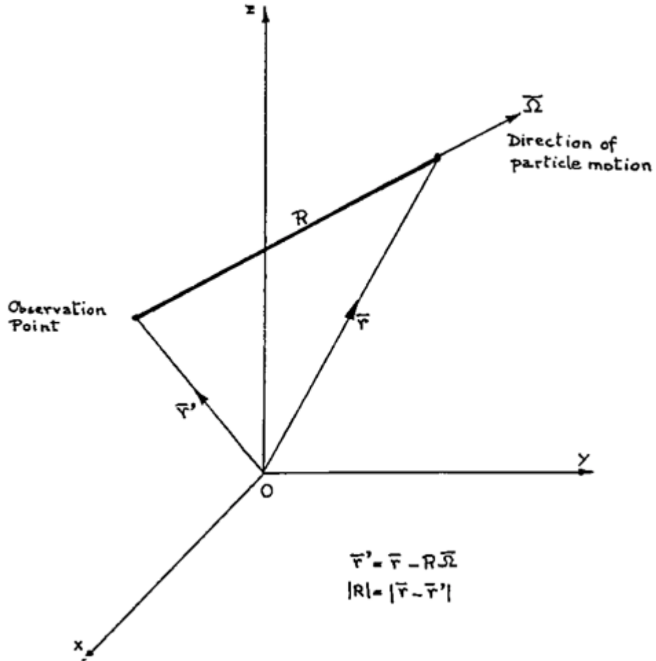
Fig. 1: Coordinate System for particle transport.
