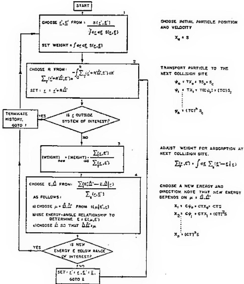
Fig. 2: Procedure for estimation of ingoing and outgoing collision densities.
